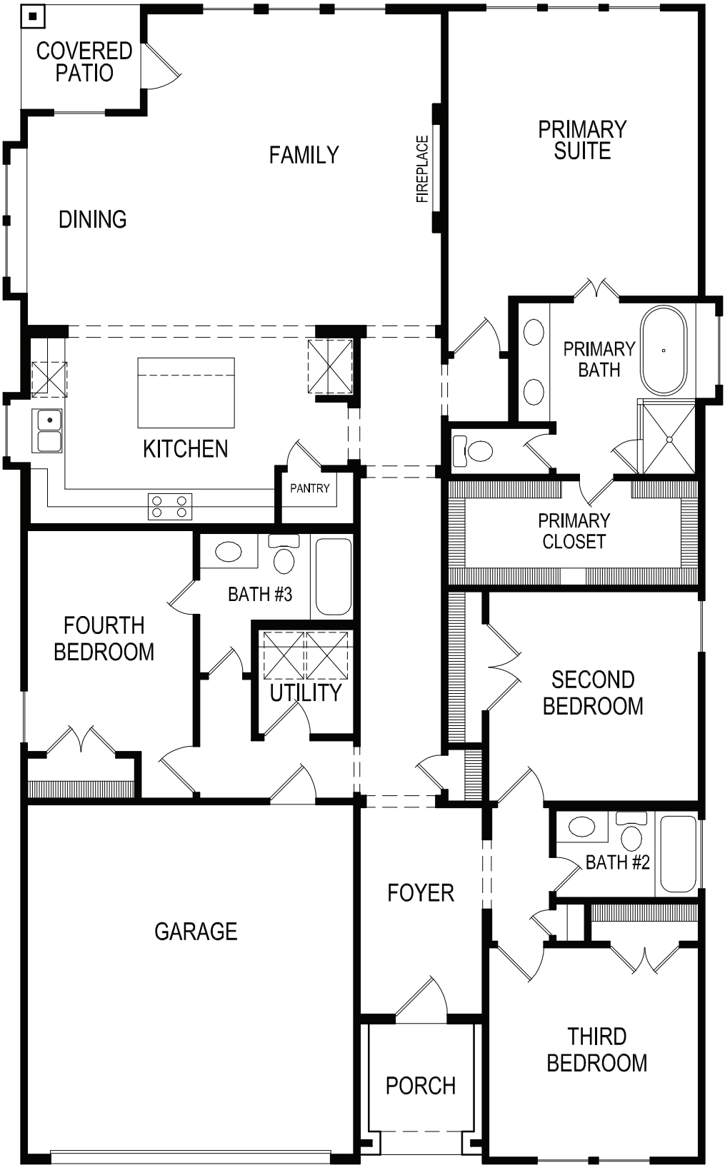
FLOOR PLAN
