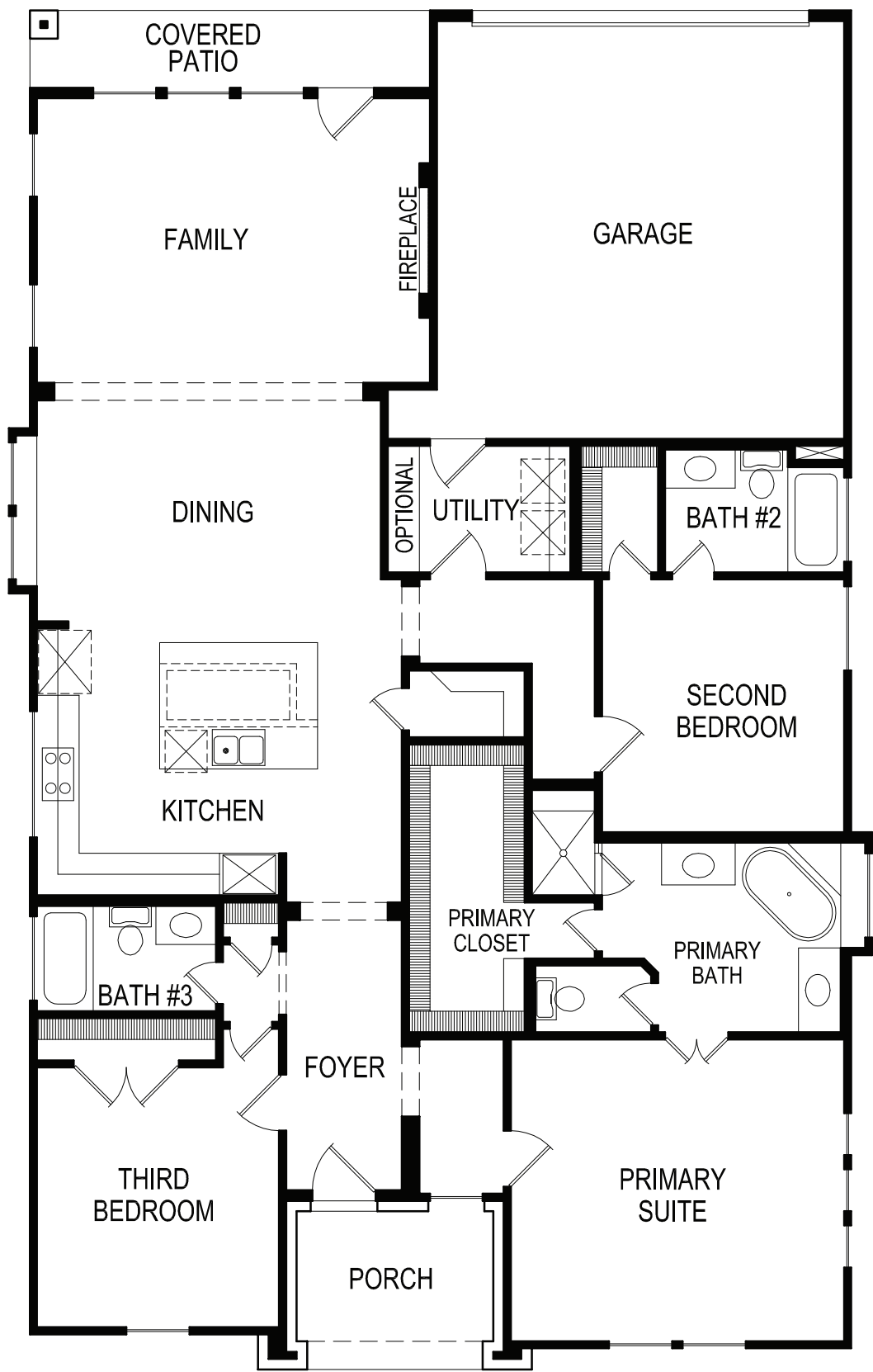
FLOOR PLAN
