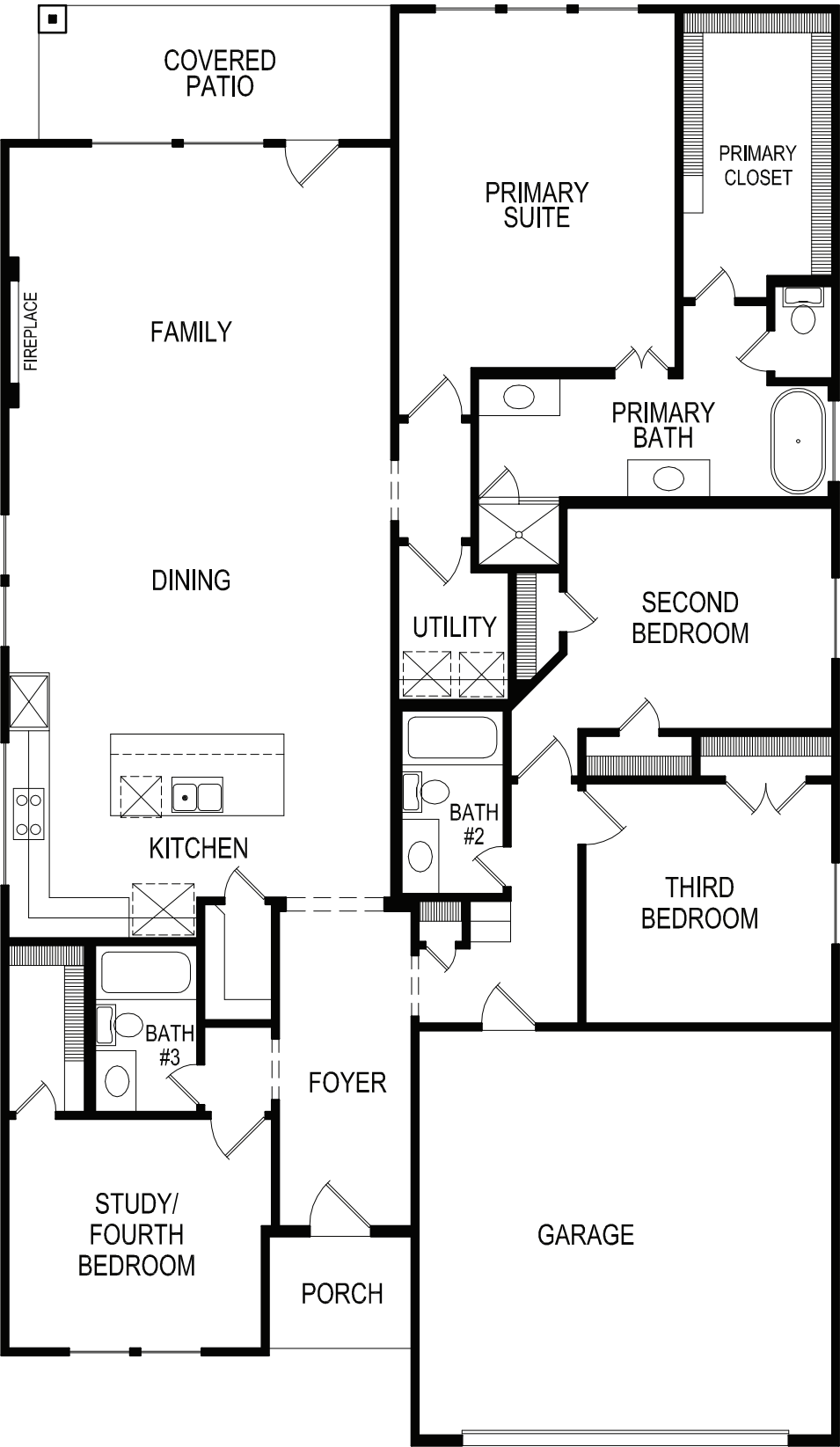
FLOOR PLAN
