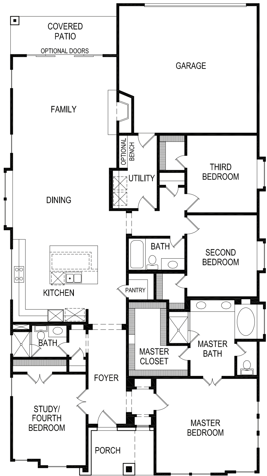
FLOOR PLAN
