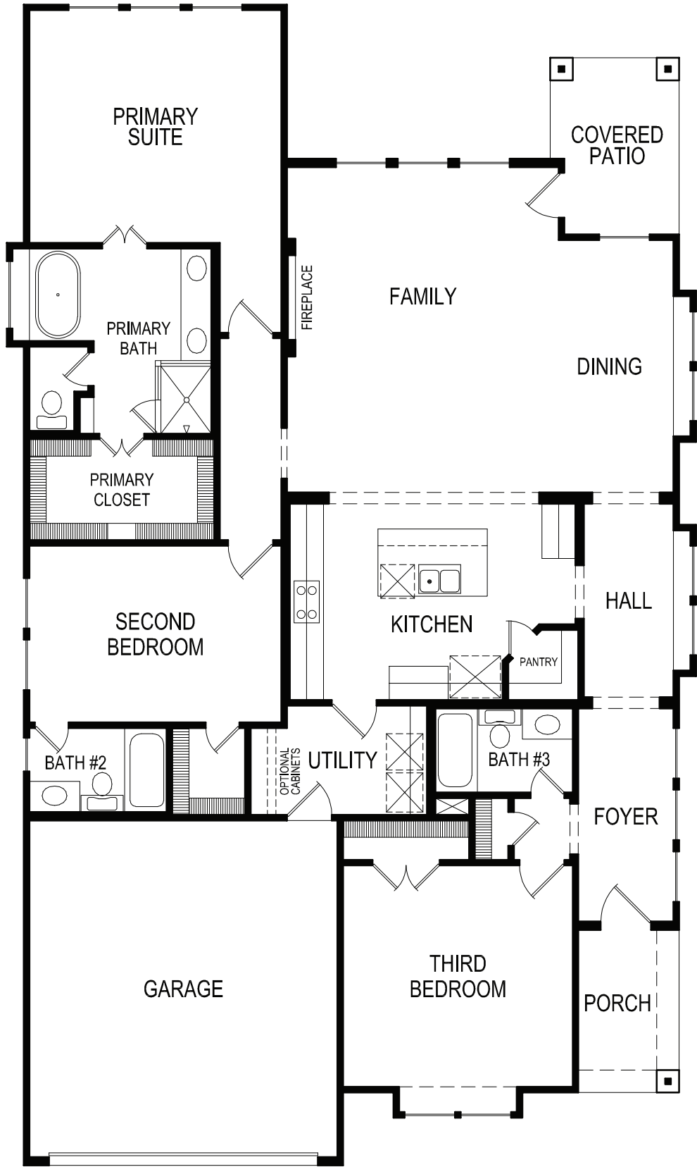
FLOOR PLAN
