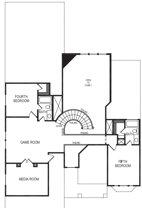
SECOND FLOOR PLAN (OPTIONAL)
